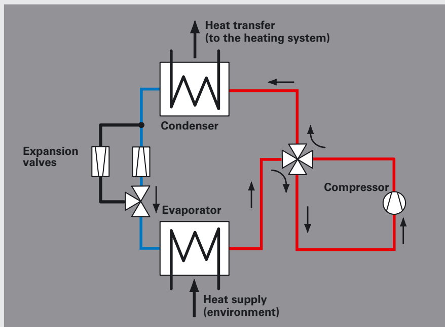
Fig. 1: Simplified function diagram for a heat pump with reversible operation in heating mode
