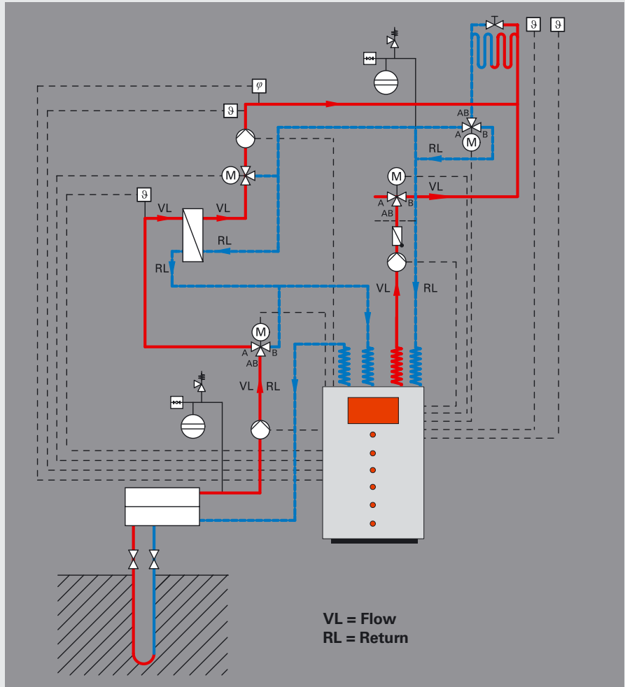
Fig. 15: Cooling with underfloor heating systems
